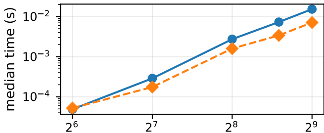
ill_conditioned | BLAS=1
