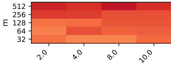
ill_conditioned | BLAS=1
