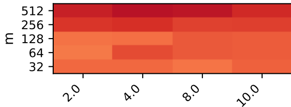
ill_conditioned | BLAS=4
