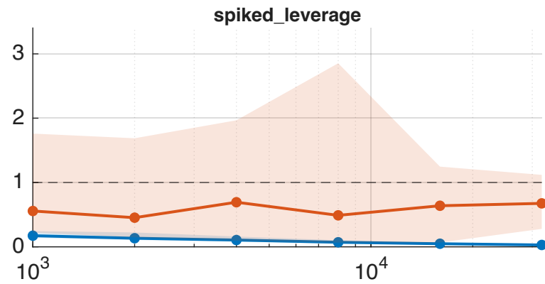
Selection quality vs bounds (m=256)
