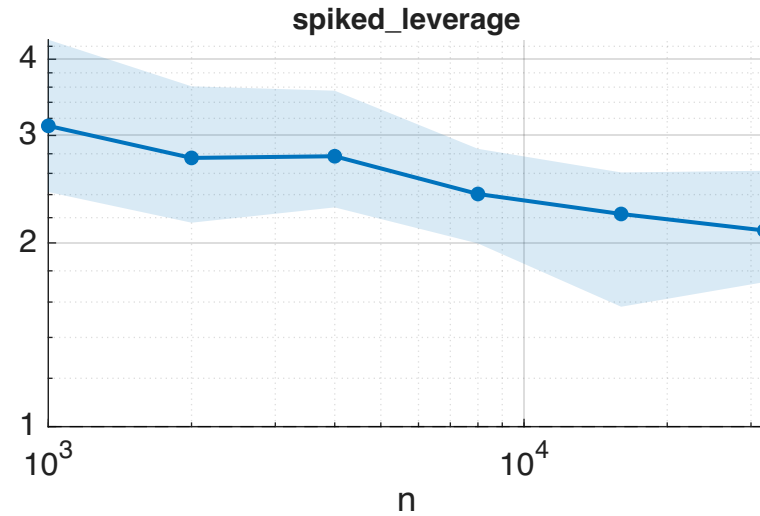
Speedup of randBSQR over rejection_rpqr (m=128)
