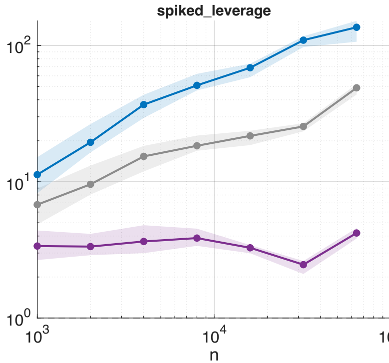
Speedup over baselines (m=64)
