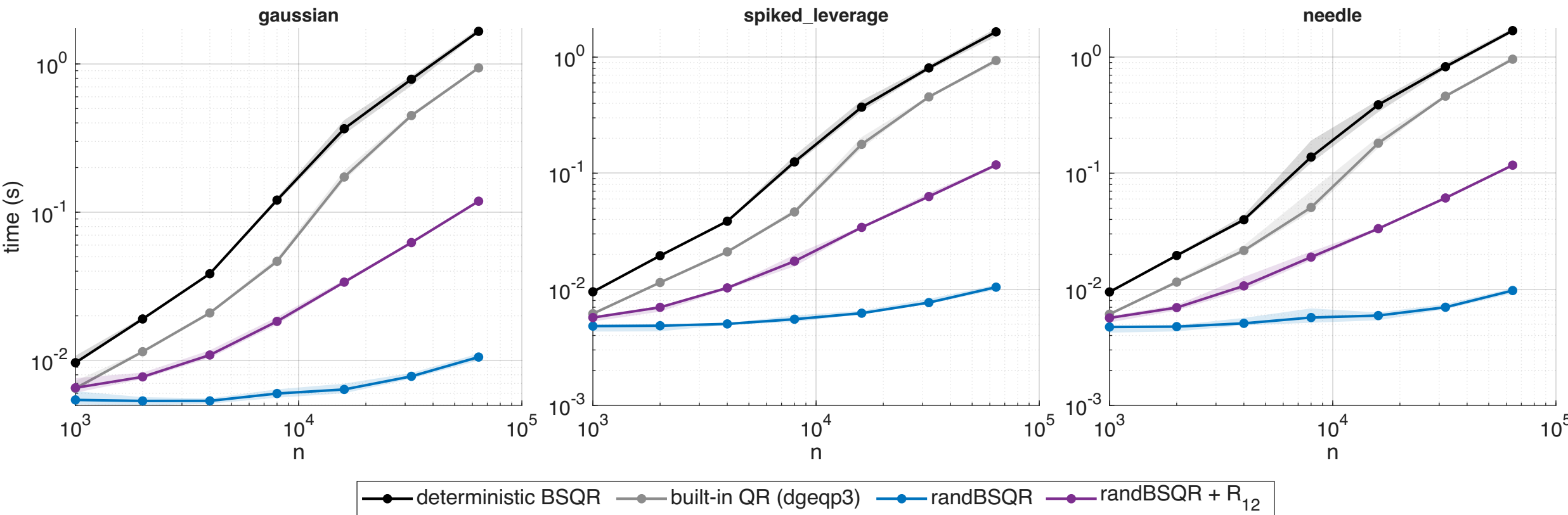
Runtime vs n ( m=256 )
