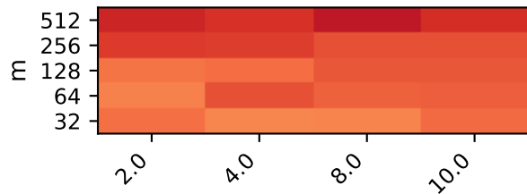
ill_conditioned | BLAS=1
