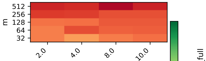
ill_conditioned | BLAS=4
