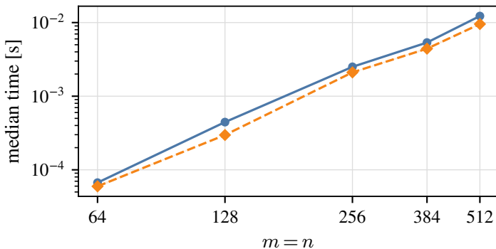
Orthonormal rows — 1 thread
