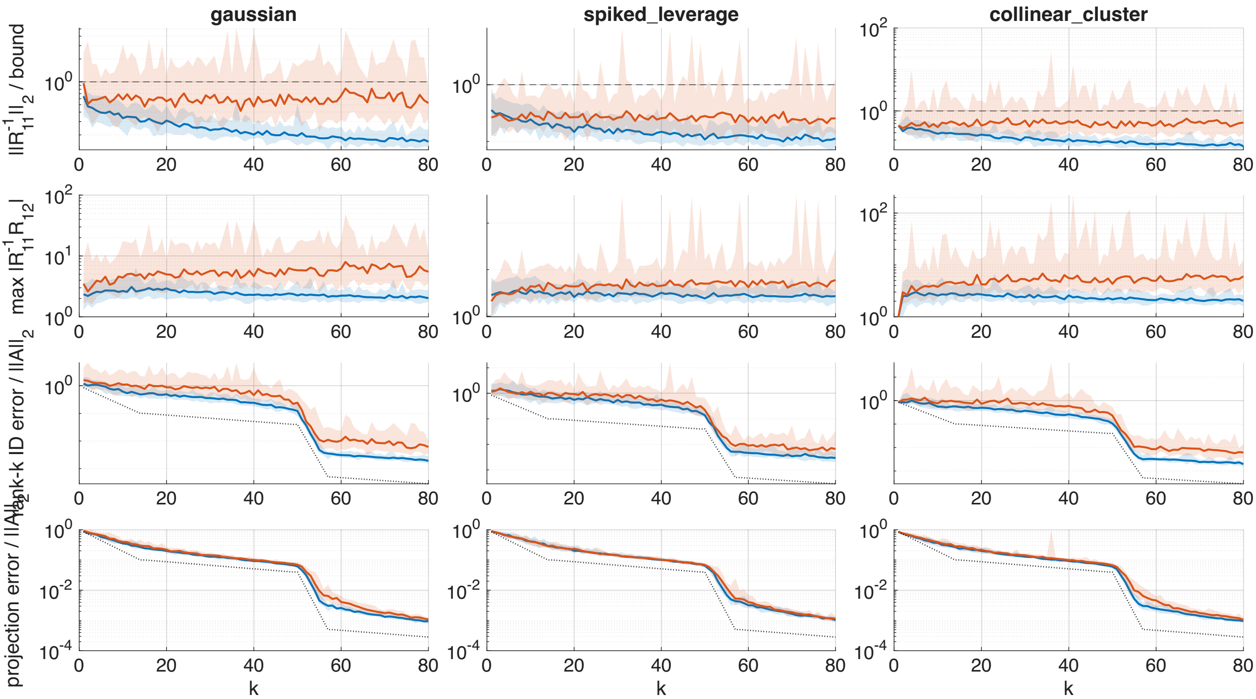
Matrix approximation quality
