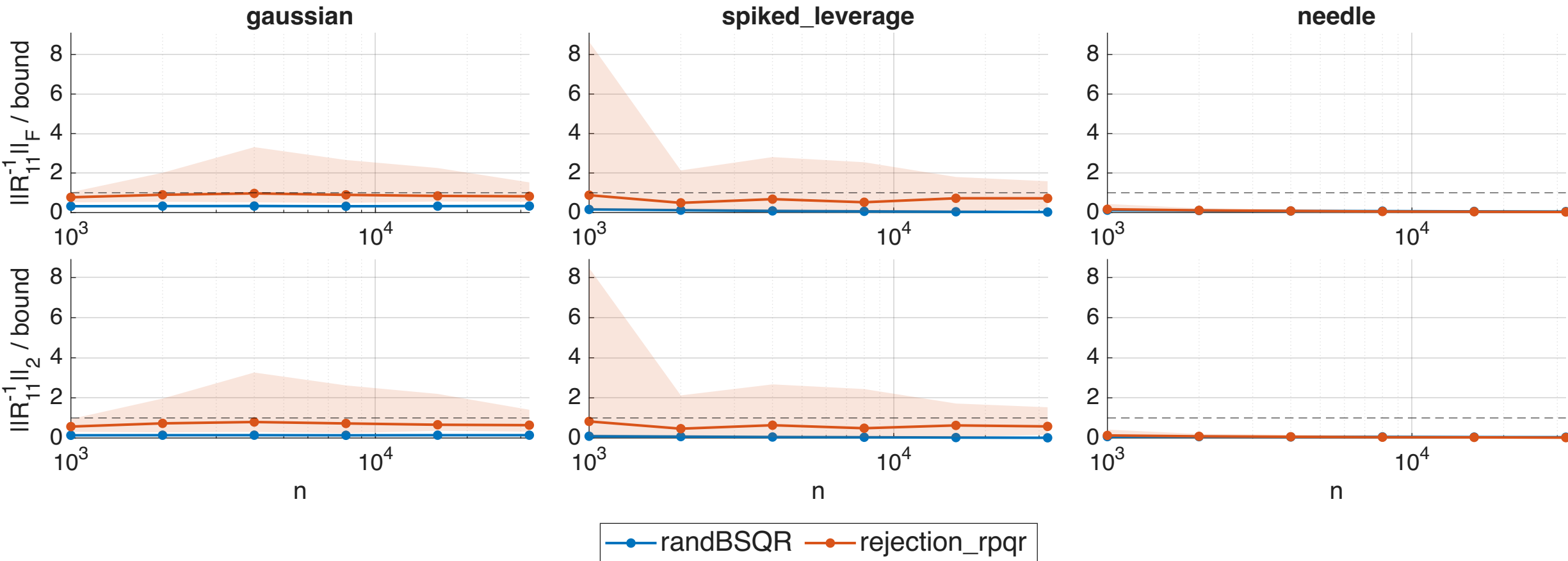
Selection quality vs bounds (m=128)
