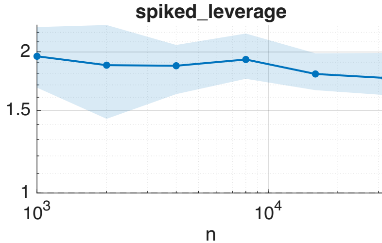
Speedup of randBSQR over rejection_rpqr (m=256)
