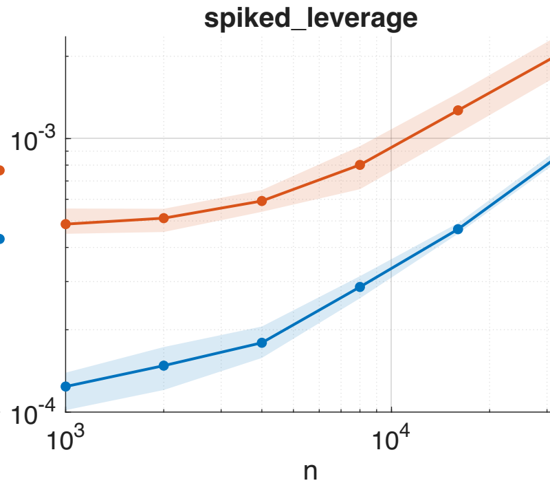
Runtime vs n (m=64)
