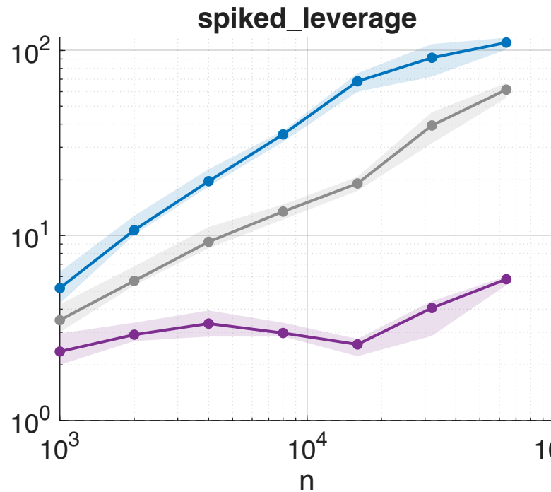
Speedup over baselines (m=128)
