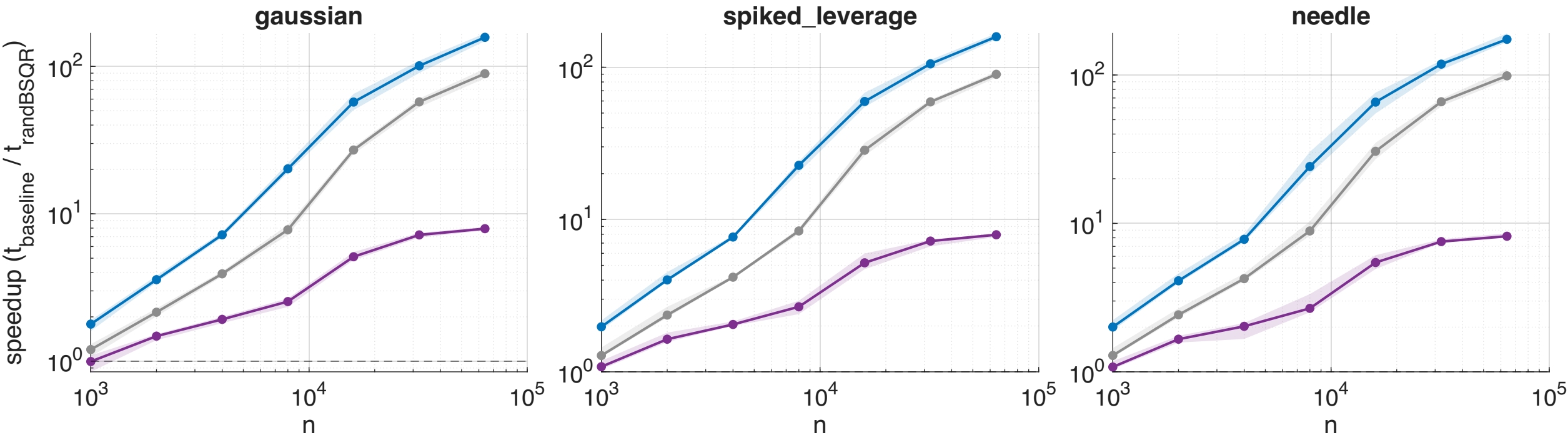
Speedup over baselines (m=256)
