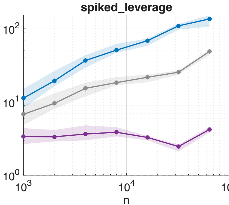
Speedup over baselines (m=64)
