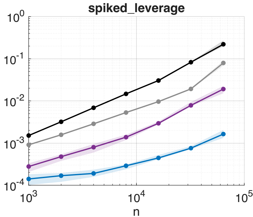
Runtime vs n (m=64)
