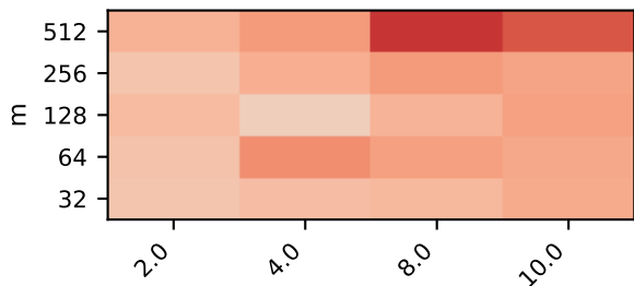
Ill-conditioned | BLAS=1
