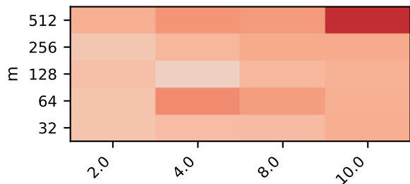
Ill-conditioned | BLAS=4
