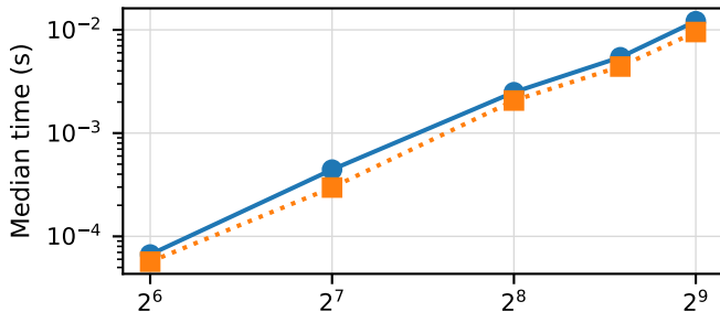
Ill-conditioned | BLAS=4
