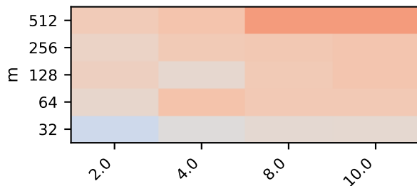
Ill-conditioned | BLAS=1
