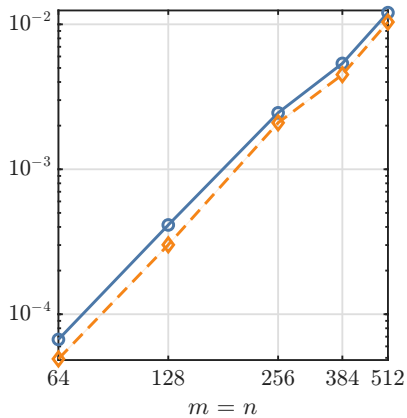
Ill-conditioned
