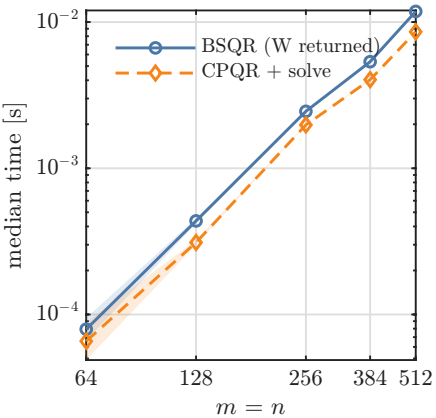
Gaussian
