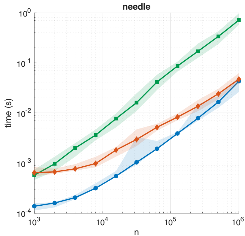
Runtime vs n at fixed m = 64
