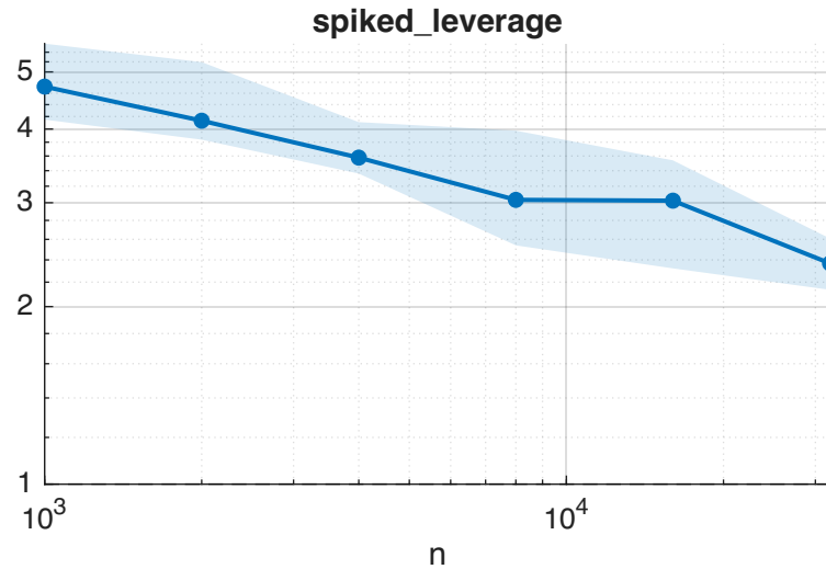
Speedup of randBSQR over rejection_rpqr (m=64)
