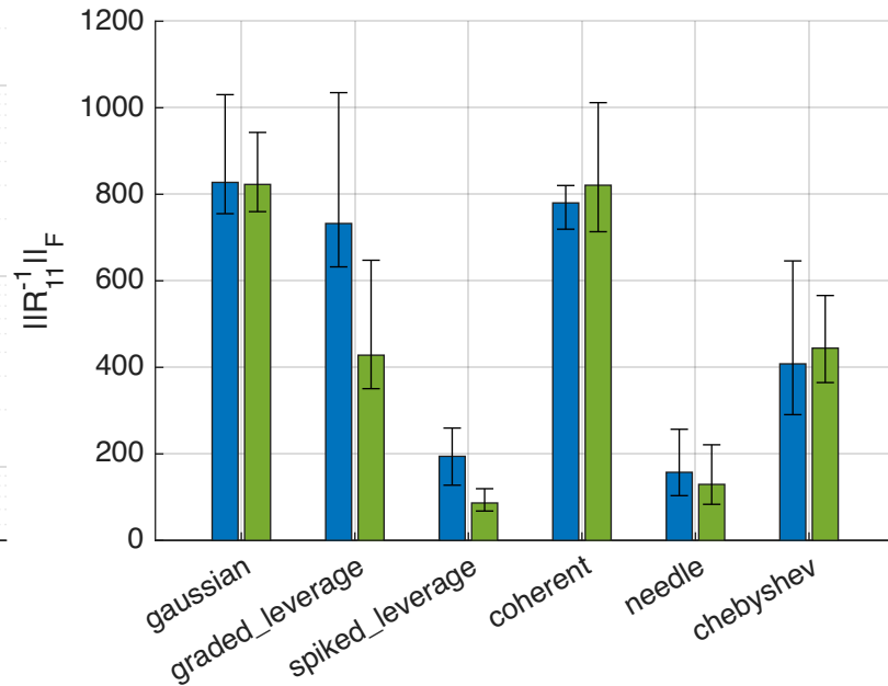
Uniform vs norm-weighted sampling ( m=256 , n=32000 , k_b=256 )
