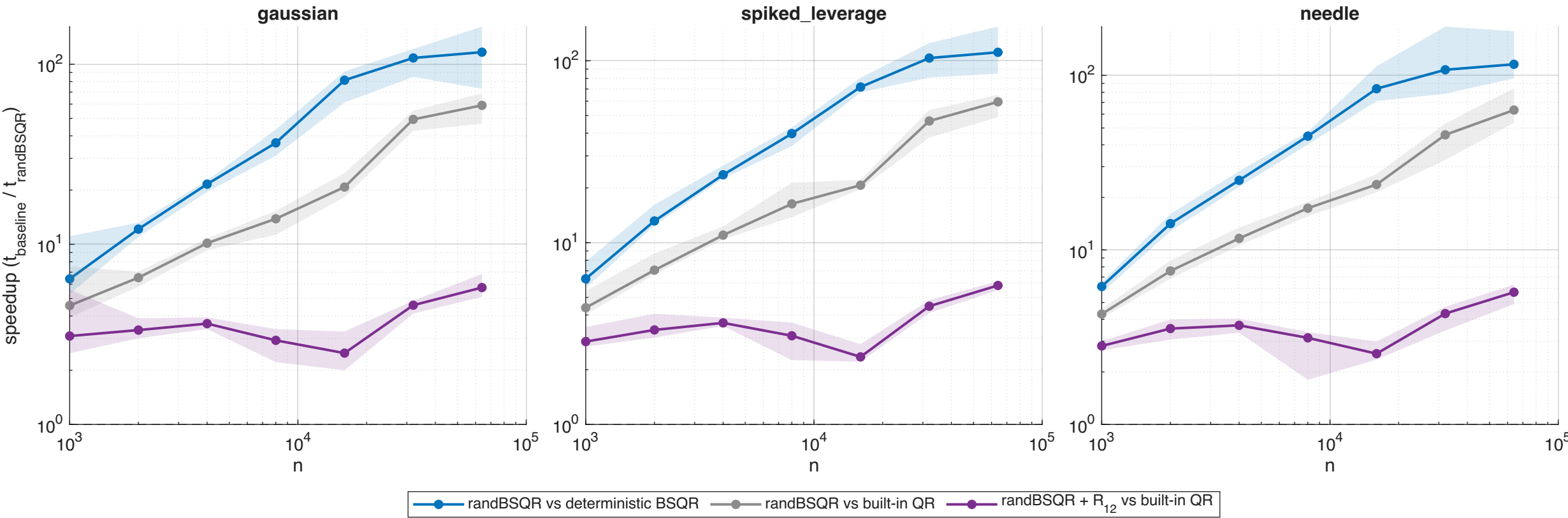
Speedup over baselines (m=128)
