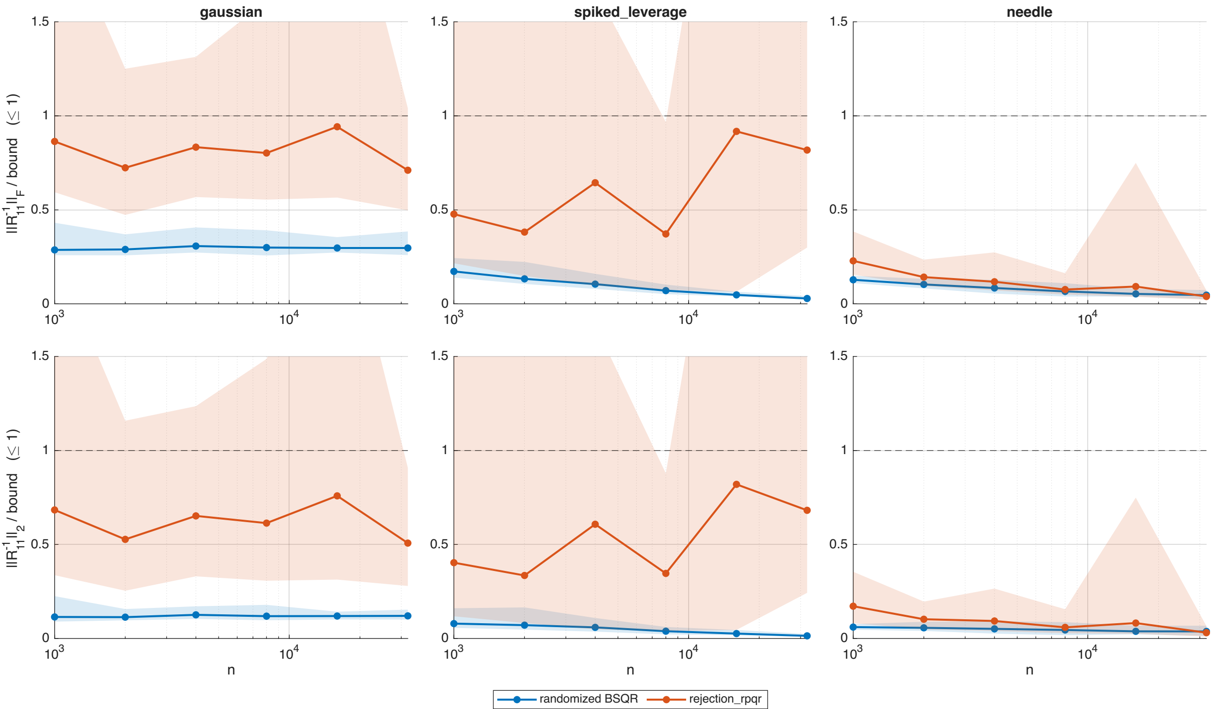
Selection quality vs the bounds (k=256, lower = better): Frobenius \|R_{11}^{-1}\|_F (top), spectral \|R_{11}^{-1}\|_2 (bottom)
