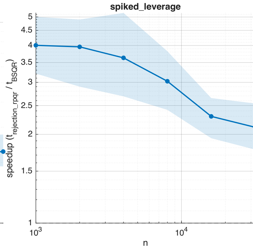
Speedup of randomized BSQR over rejection_rpqqr ( t_{\text{rpqr}}/t_{\text{BSQR}} ) ( k=128 )
