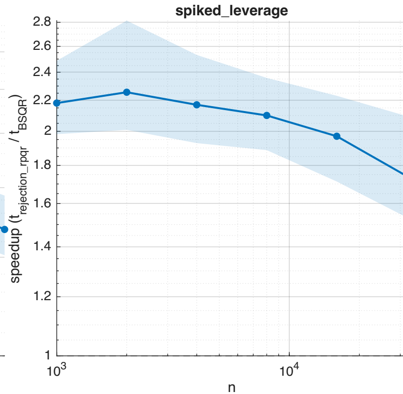
Speedup of randomized BSQR over rejection_rpq (t rpqr /t BSQR ) (k=256)
