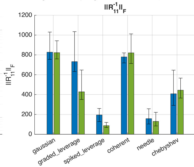
Uniform vs norm-weighted sampling across families (k=256, n=32000, block=256)
