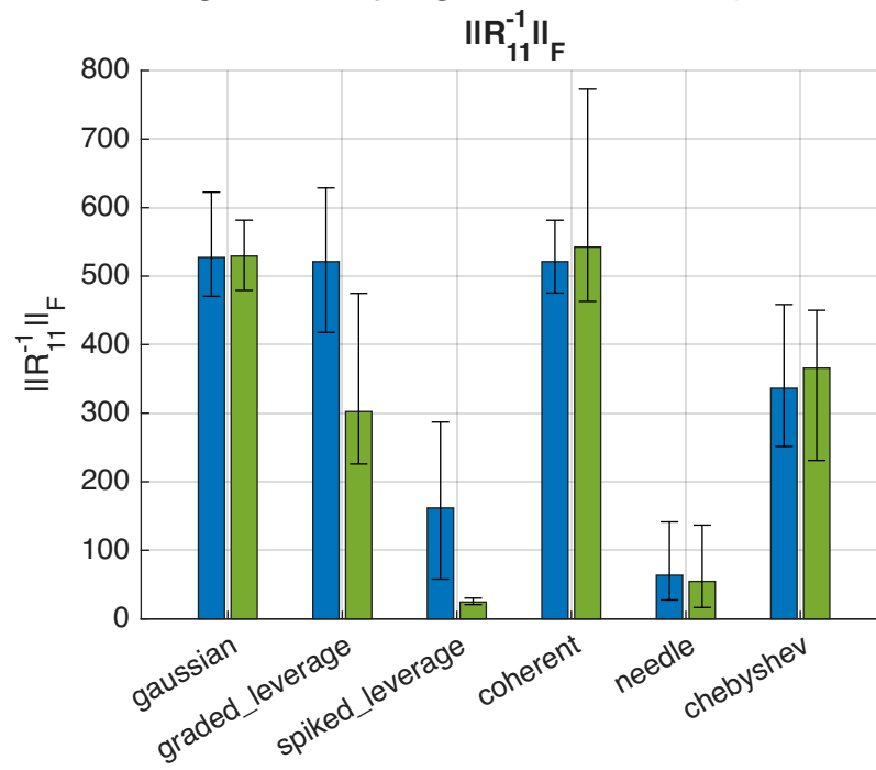
Uniform vs norm-weighted sampling across families (k=64, n=32000, block=64)
