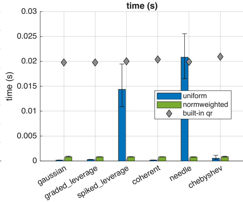
Uniform vs norm-weighted sampling across families (k=64, n=32000, block=64)
