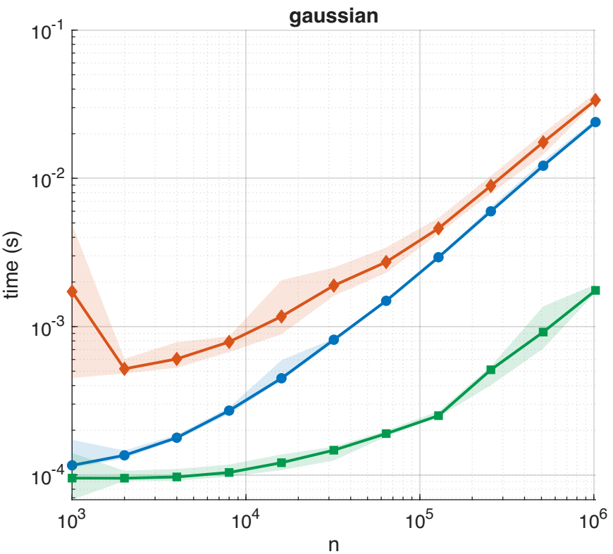
Runtime vs n at fixed k = 64
