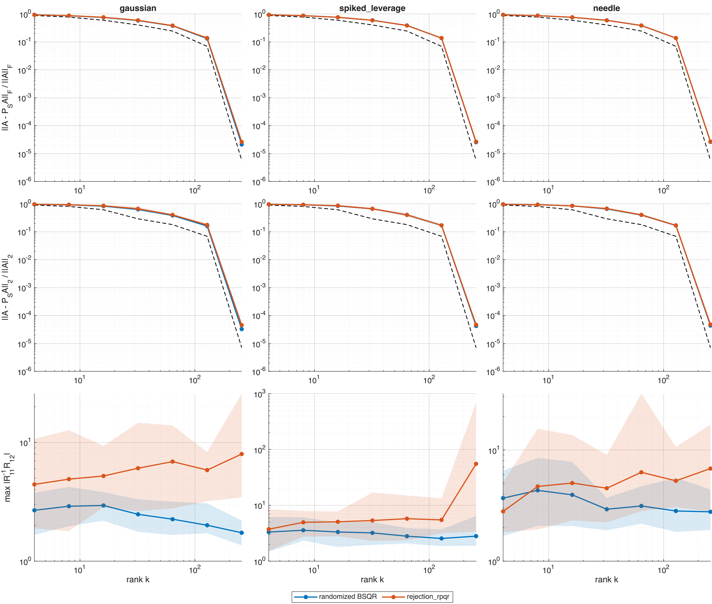
Approximation accuracy vs interpolation coefficients (vs rank k): Frobenius / spectral error (top two, dashed = optimal rank-k), \max |R_{11}^{-1} R_{12}| (bottom)
