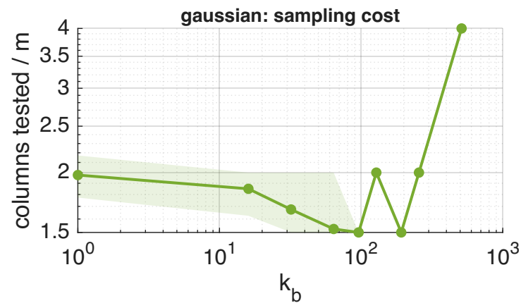
Effect of block size on norm-weighted sampling ( m=128 )
