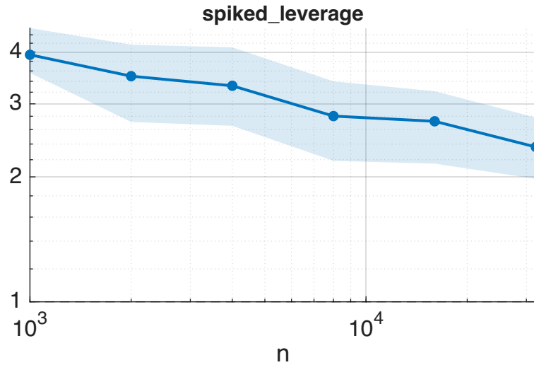
Speedup of randBSQR over rejection_rpqr (m=64)
