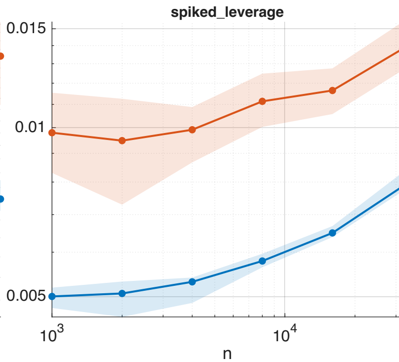
Runtime vs n (m=256)
