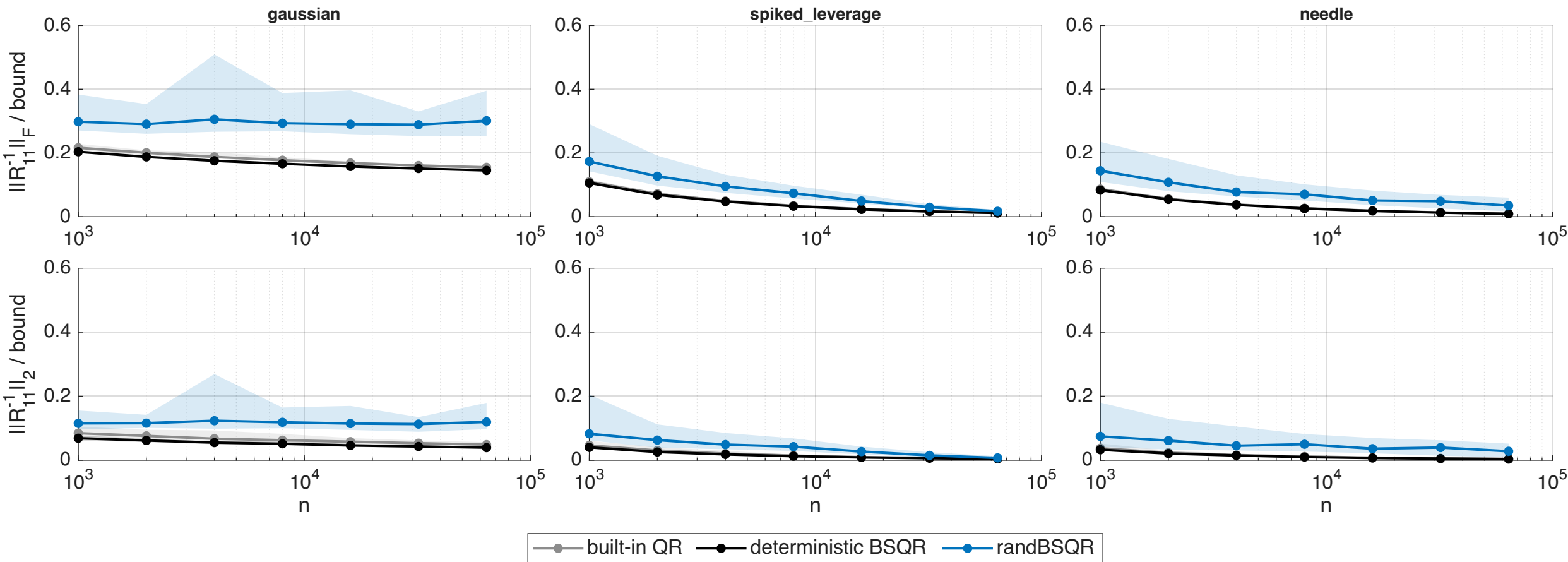
Selection quality vs bounds (m=256)
