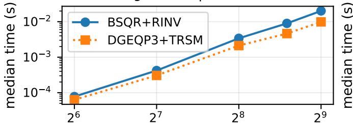
ill_conditioned | BLAS=1
