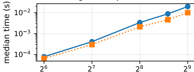
ill_conditioned | BLAS=4
