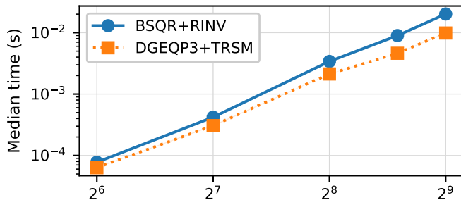
Ill-conditioned | BLAS=1
