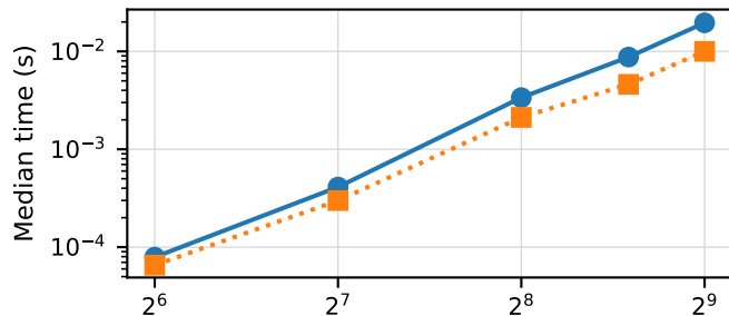
Ill-conditioned | BLAS=4
