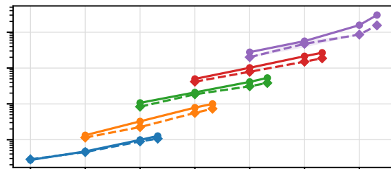
Gaussian — 4 threads
