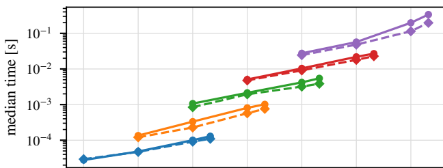
Ill-conditioned — 1 thread
