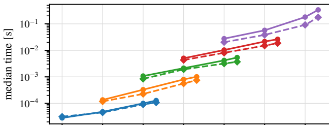
Gaussian — 1 thread
