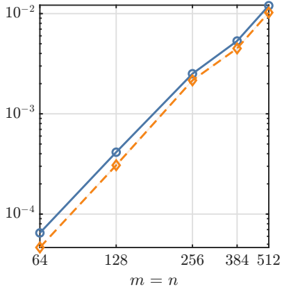
Ill-conditioned
