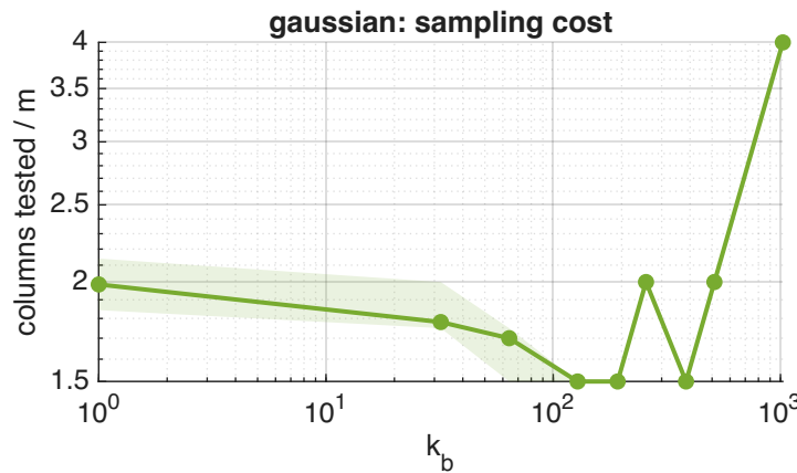
Effect of block size on norm-weighted sampling ( m=256 )
