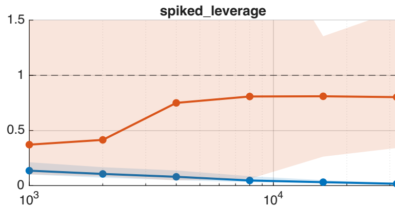
Selection quality vs bounds (m=64)
