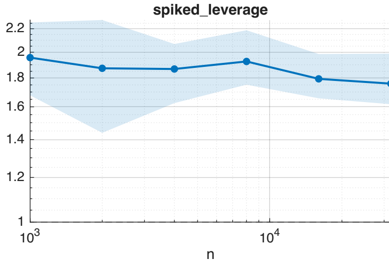
Speedup of randBSQR over rejection_rpqr (m=256)
