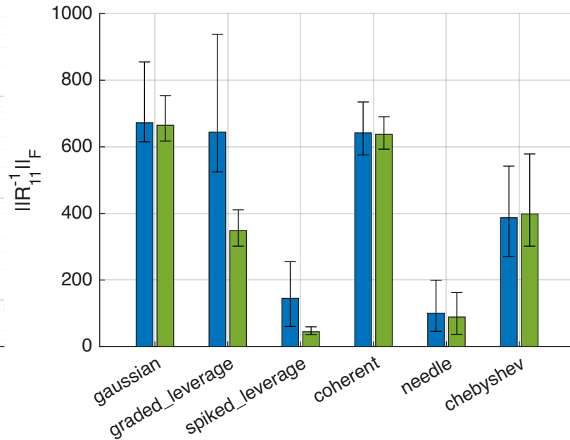
Uniform vs norm-weighted sampling ( m=128 , n=32000 , k_b=128 )
