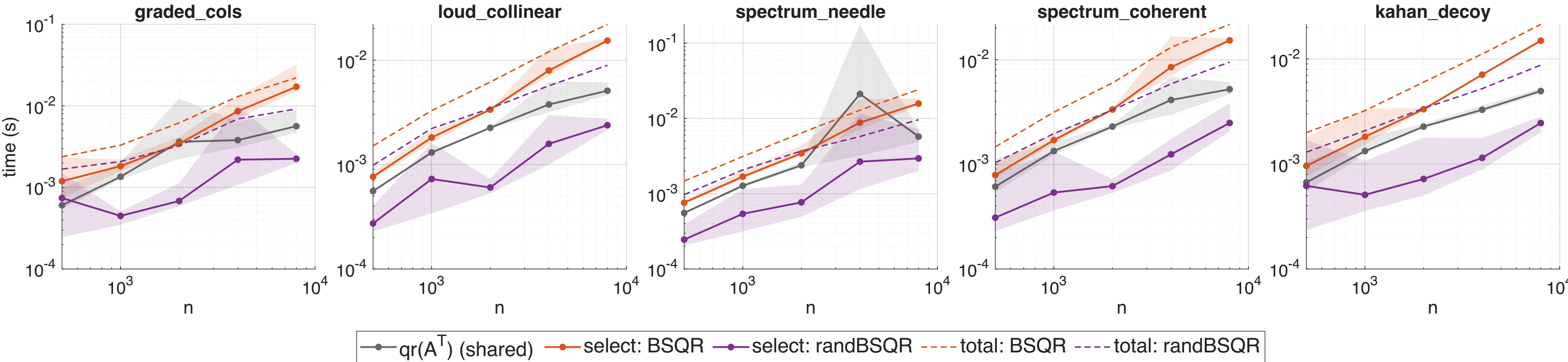
bsqr_general phase split vs n (m = k = 64)
