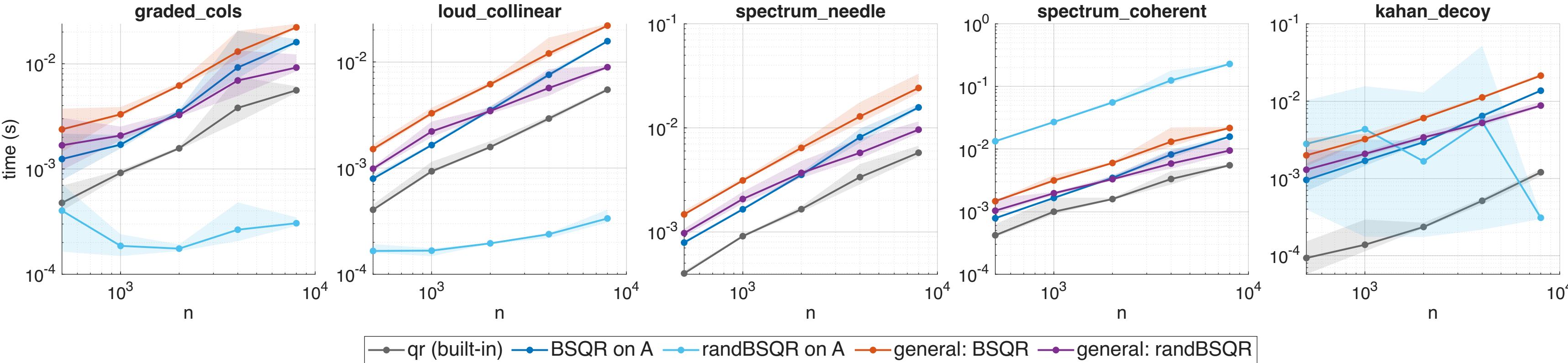
Runtime vs n ( m = k = 64 )
