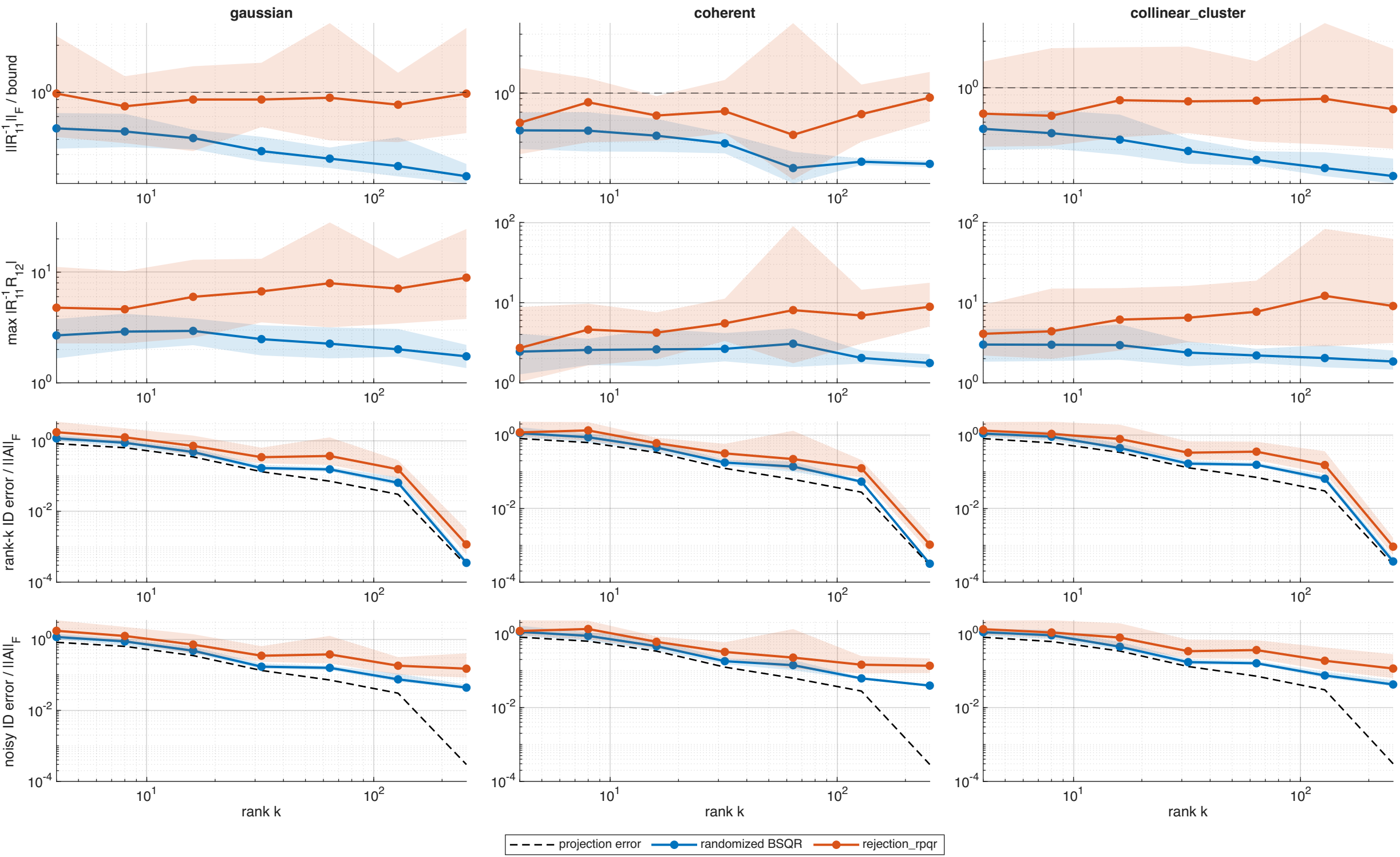
\|IR_{11}^{-1}\| matters (Frobenius norm): conditioning, coefficients, rank-k ID error (noiseless vs noisy (noise \epsilon=1e-02 )); dashed = projection optimum
