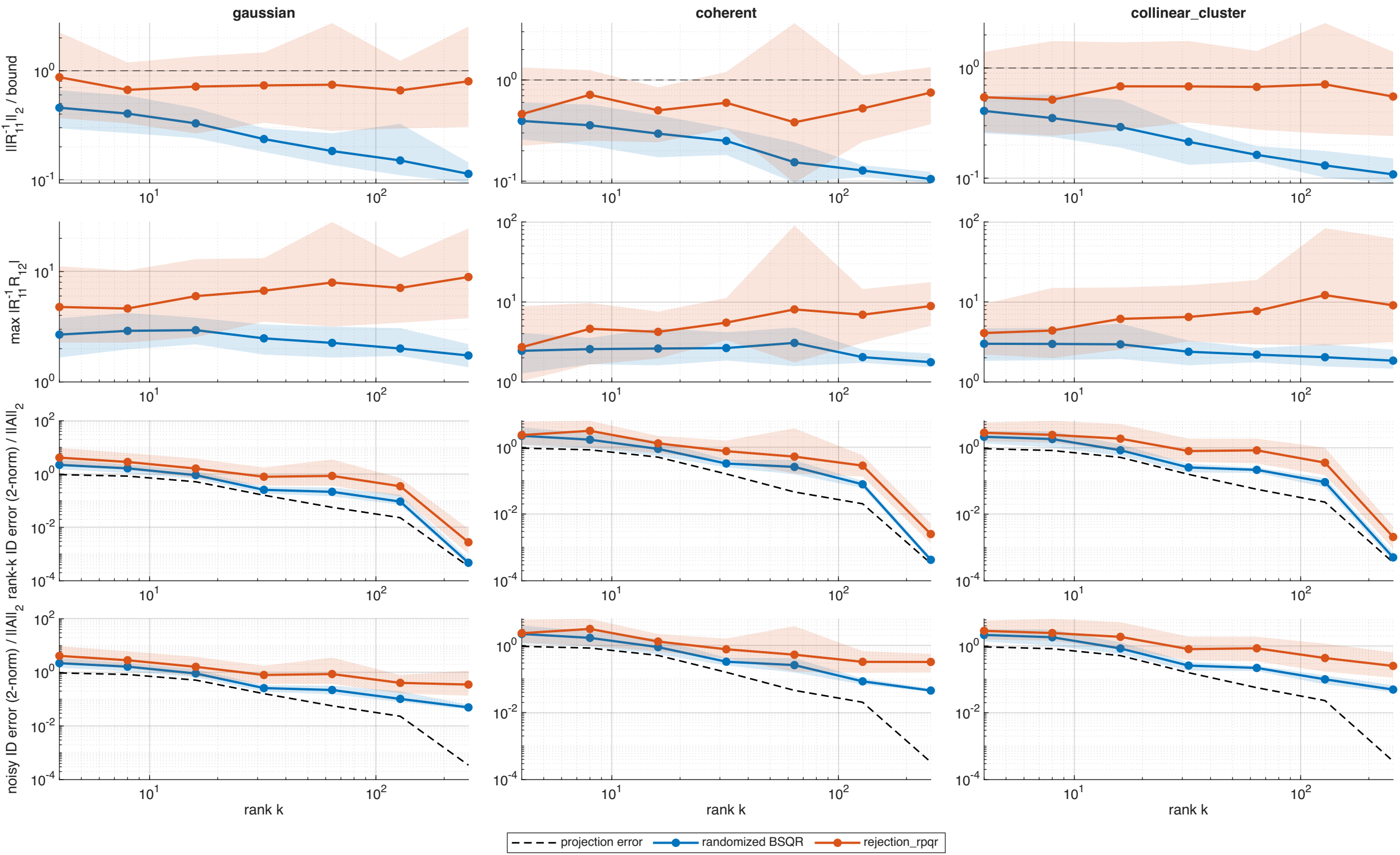
\|R_{11}^{-1}\| matters (spectral norm): conditioning, coefficients, rank-k ID error (noiseless vs noisy (noise \epsilon=1e-02 )); dashed = projection optimum
