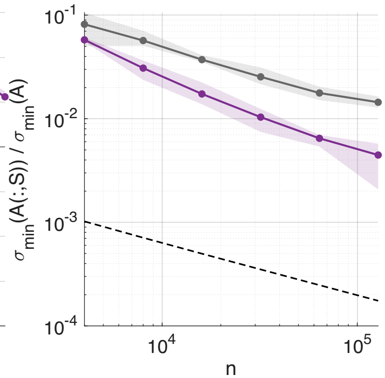
Built-in pivoted QR vs general randBSQR (graded_cols, m = k = 256 )
