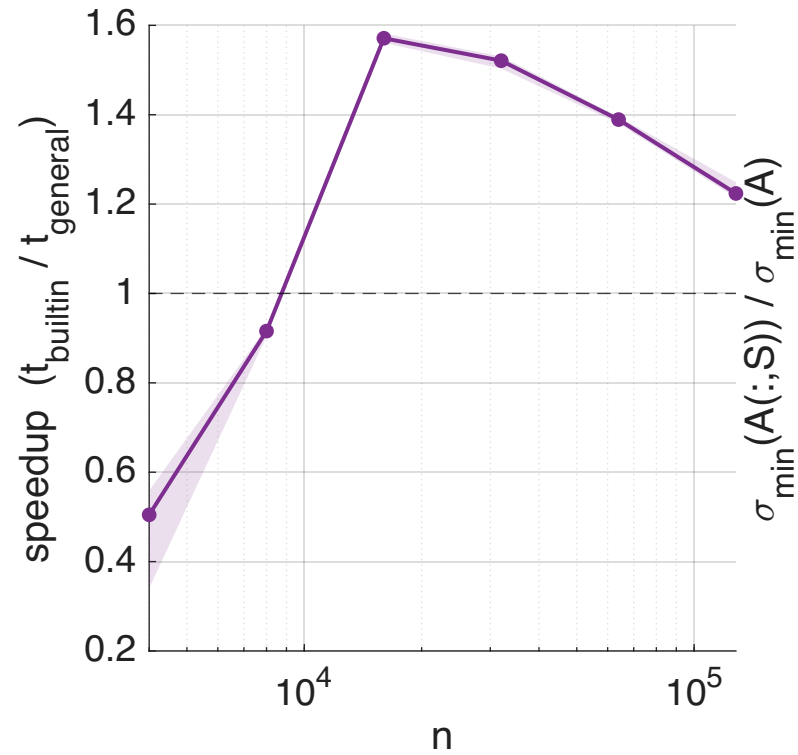
Built-in pivoted QR vs general randBSQR (graded_cols, m = k = 256 )
