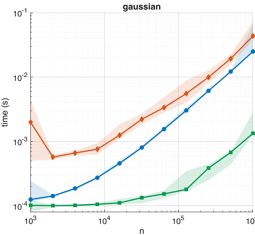
Runtime vs n at fixed k = 64
